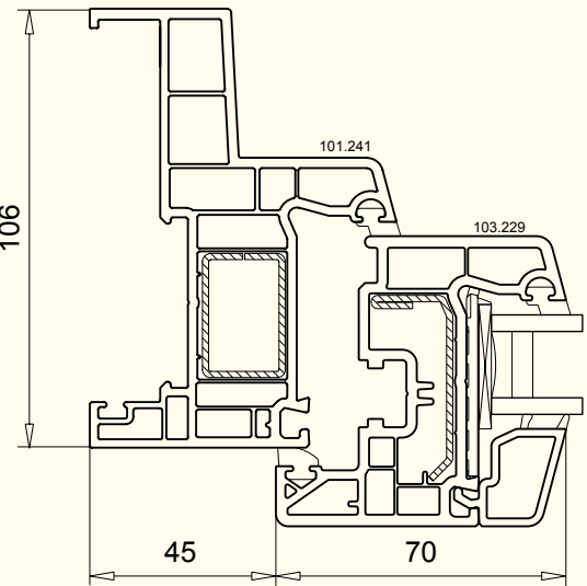
OptiLine VEKA 70 WITH INSULATION FRAME
